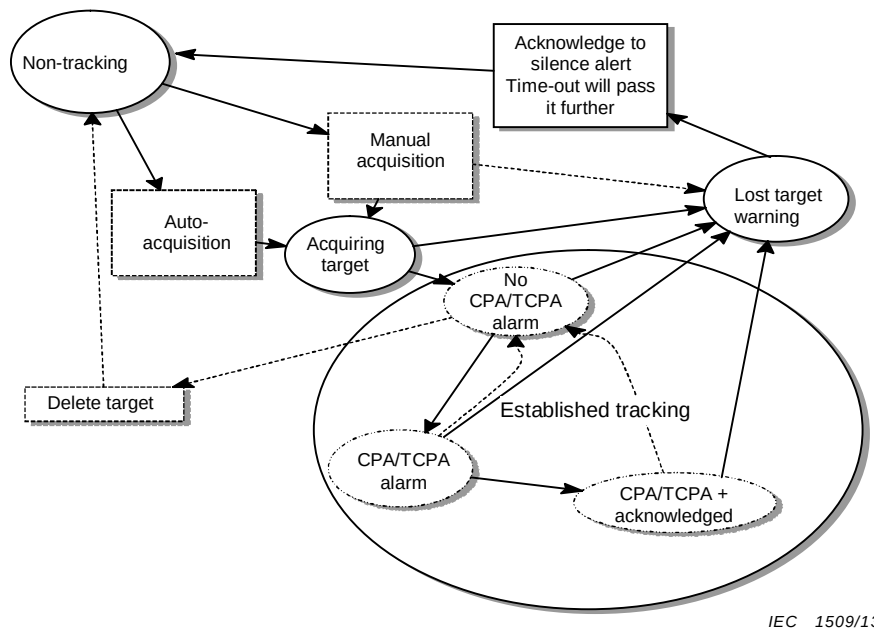
Figure G.1 – Tracked target states
