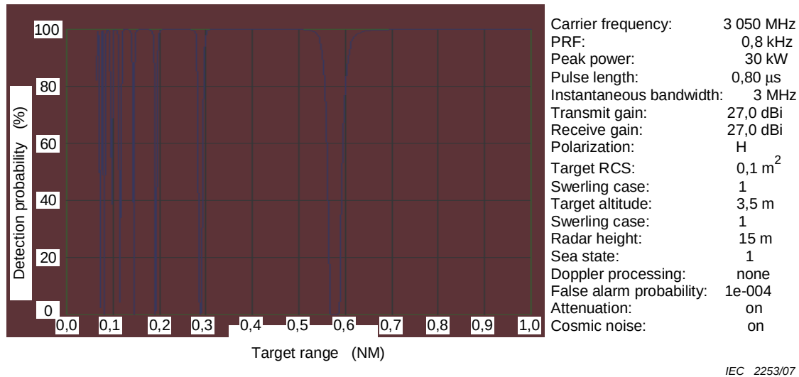
Figure D.2 – Multi-path plots for S-band
